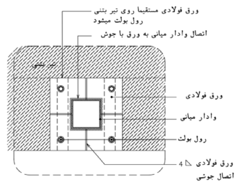
Det.2 sec.C-C
